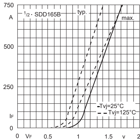
Fig.15 Forward characteristics
