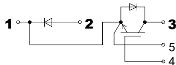
SDG150T120UC2
