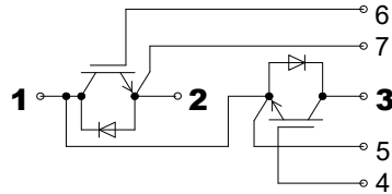
SDG150T120UC2
