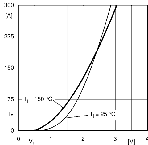
Fig. 10: Typ. FRD diode forward charact., incl. R_{CC} + EE'
