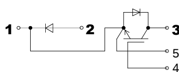
SDG145T60UC1 (Buck Chopper)
