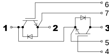
SDG145T60UC1 (Buck Chopper)
