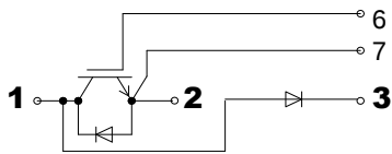
SGD145T60UC1 (Boost Chopper)
