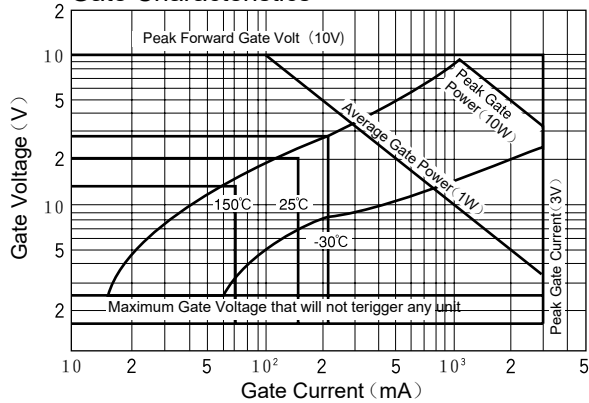
Gate Characteristics
