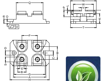
Dimensions SOT-227(ISOTOP)
