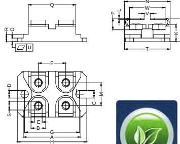
Dimensions SOT-227(ISO TOP)
