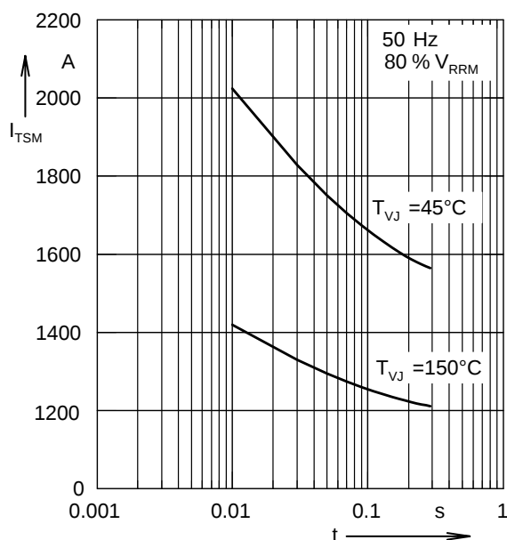
Fig.4 Surge overload current
