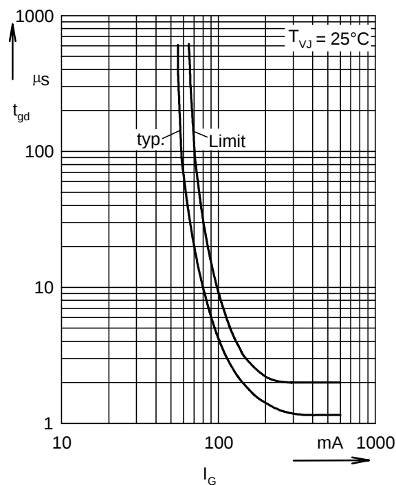
Fig. 2 Gate trigger delay time
