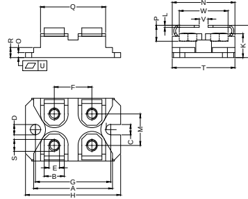
Dimensions SOT-227(ISOTOP)
