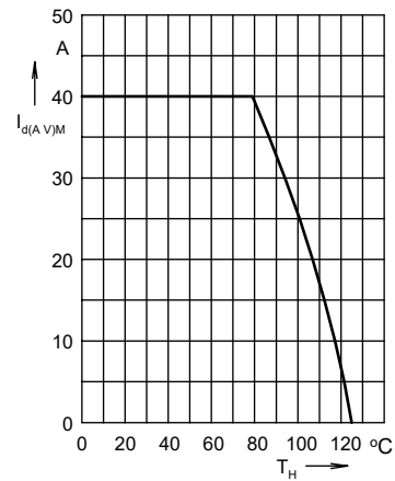
Fig. 7 Max. forward current versus heatsink temperature
