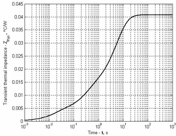
Fig 6 Transient thermal impedance junction to case Z_{thjc} per arm for DC
