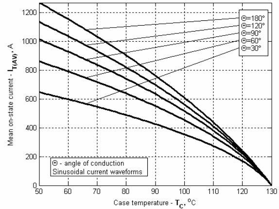
Fig 2 Mean on-state current I_{TAV} vs. Case temperature T_C for sinusoidal current waveforms at different conduction angles, f=50\text{Hz}
