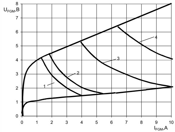
Fig 7 Gate characteristic
