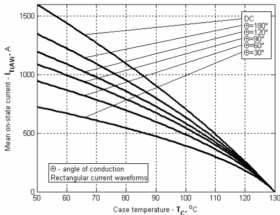
Fig 3 Mean on-state current I_{TAV} vs. Case temperature T_C for rectangular current waveforms at different conduction angles and for DC, f=50\text{Hz}
