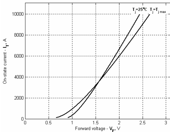
Fig 1 On-state characteristics
