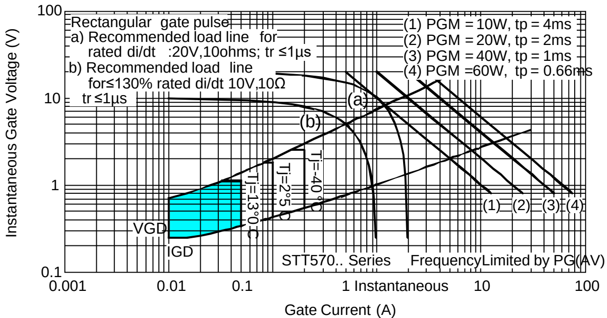
Fig. 12 - Gate Characteristics
