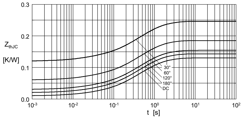
Fig. 9 Transient thermal impedance junction to case at various conduction angles
