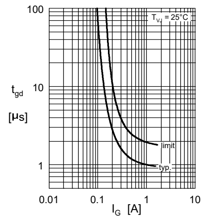
Fig. 7 Gate trigger delay time
